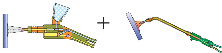
spraying powder
